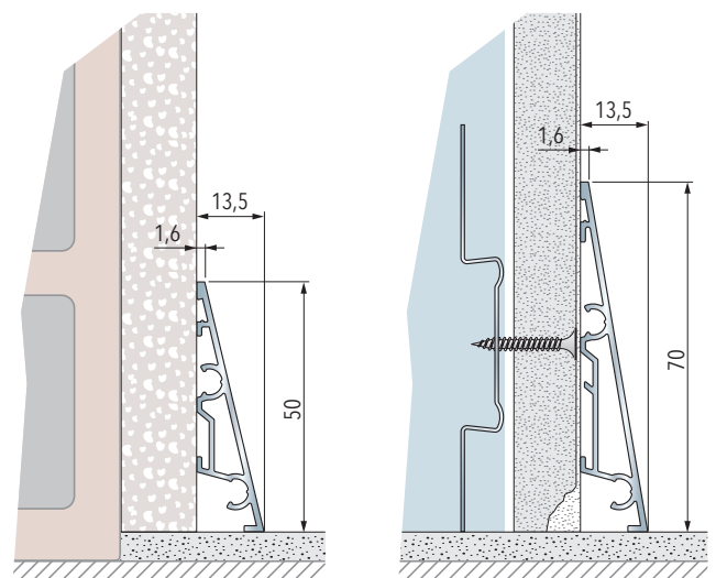
Baseboard installed on solid wall
